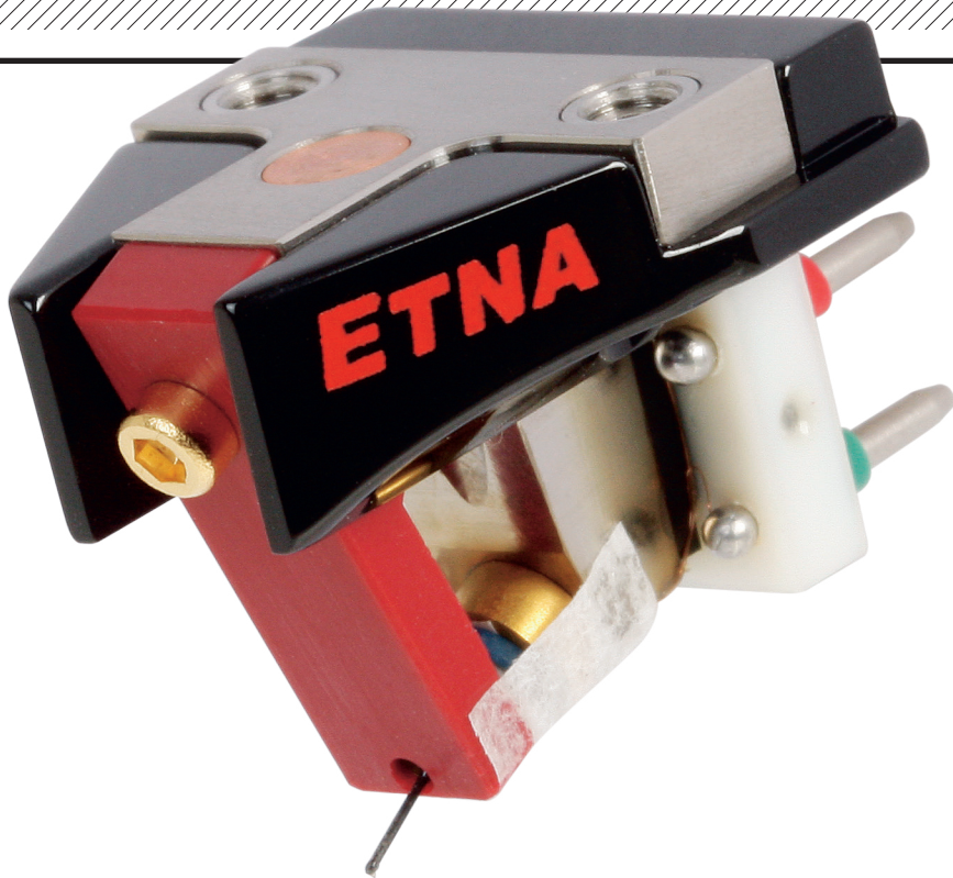
LEFT: The multi-part (titanium, duralumin, bronze and stainless steel) main body offers a rigid clamping surface and good damping. The exposed boron cantilever, while demanding caution in use, makes precise cueing very easy
